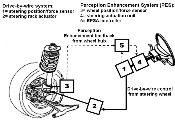
Figure 1: A perception enhancement system for use with "by-wire" automotive steering.
